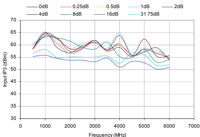
Figure 26. Input IP3 vs. Frequency
