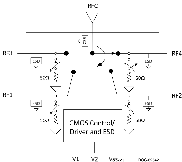
Figure 1. Functional Diagram
